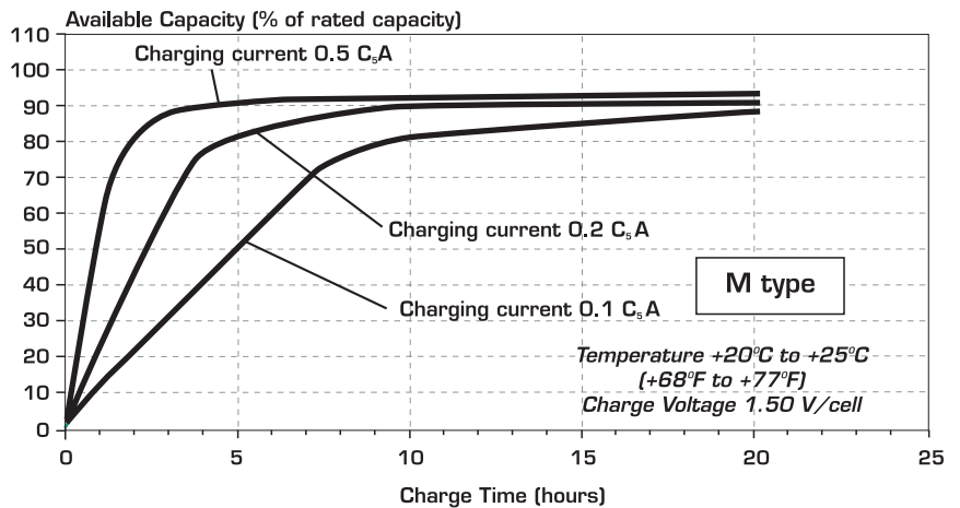
Figure 6(d) - Typical recharge times for different charge rates for the M block
