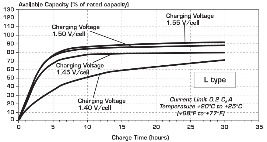
Figure 6(a) - Typical recharge times from a fully discharged state for the L block
