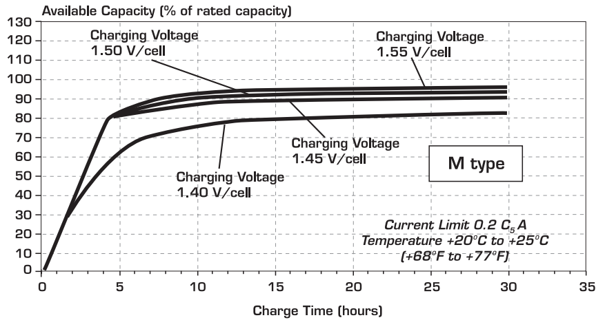
Figure 6(b) - Typical recharge times from a fully discharged state for the M block
