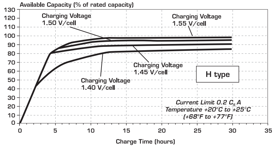
Figure 6(c) - Typical recharge times from a fully discharged state for the H block
