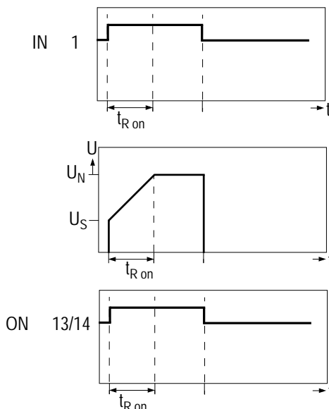
Figure 12-1 State diagram of the ON output contact
